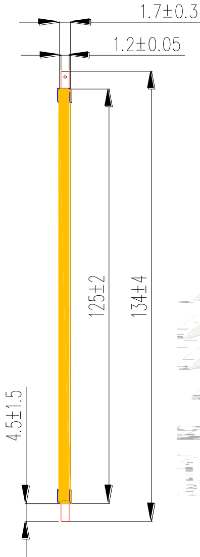
Fig.1-1 Top view
