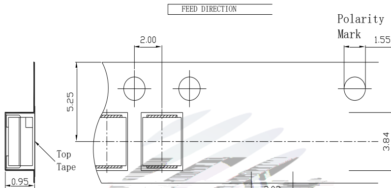
Fig.2-1 Carrier Tape Dimension
