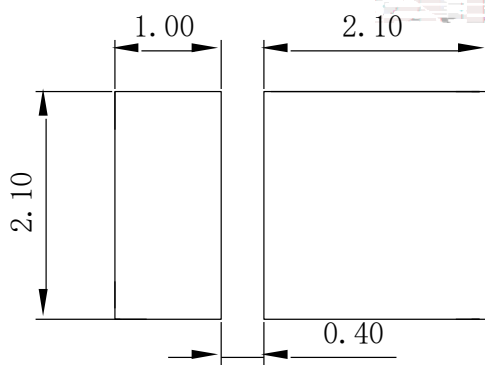
Fig.1-5 Soldering patterns
